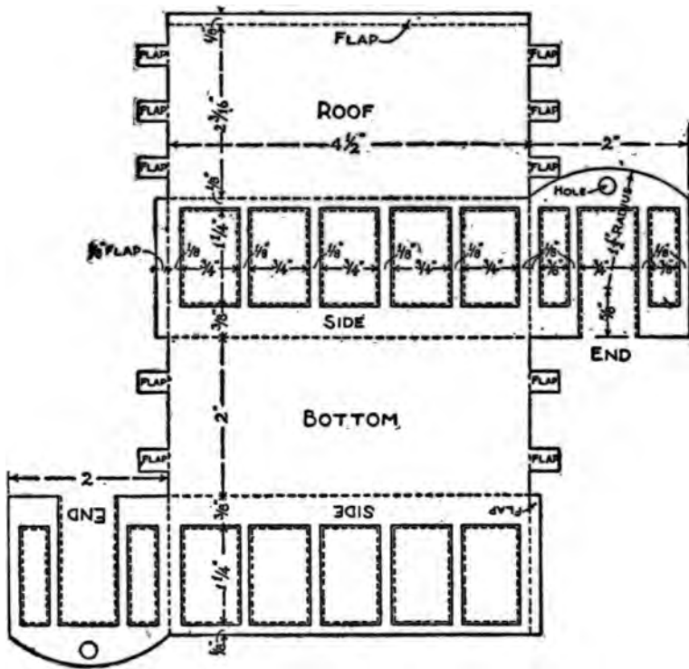
FIG. 158. — Pattern for the Ferris Wheel Cars.
